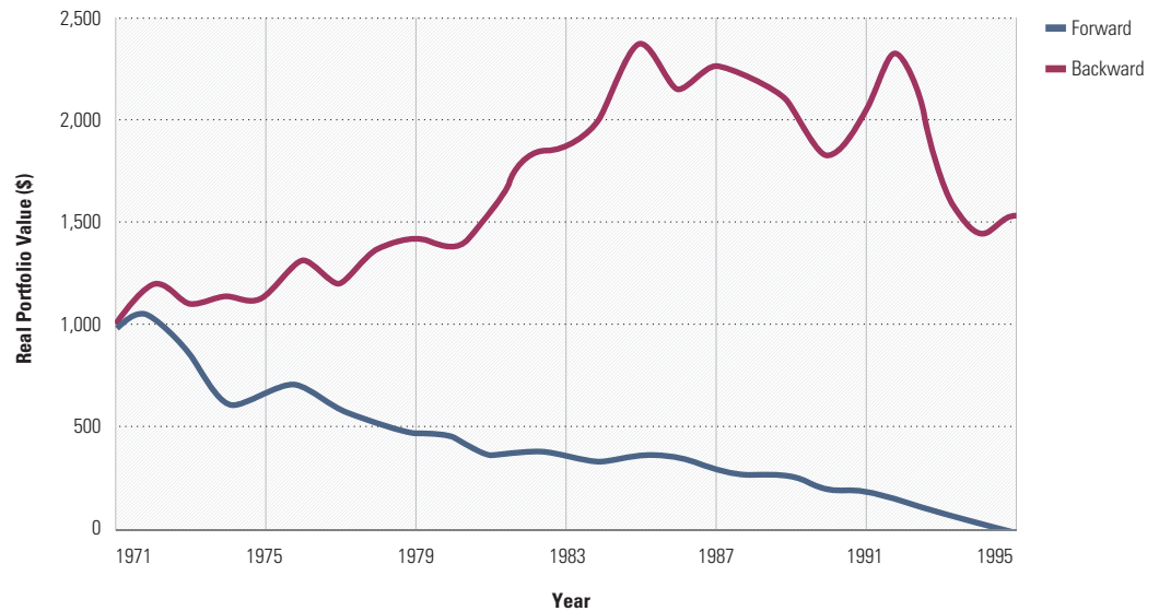
Figure 4: Sequence Risk
